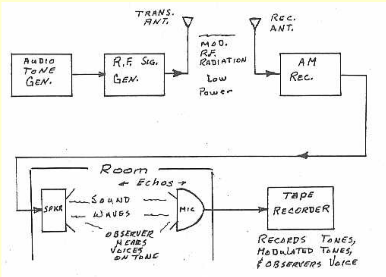
Fig. 11 Functional Block Diagram of Mark IV
